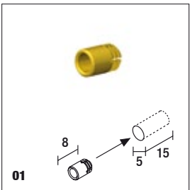
Manchon laiton Brass sleeve
